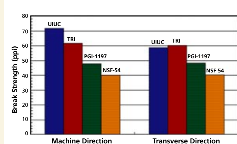
Figure 1. Tensile break strengths in the machine and transverse directions compared to NSF-54 and PGI-1197 specifications.
