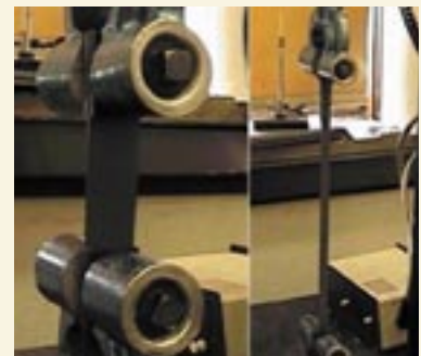
Photo 2: Exhumed PVC before and during tensile testing.
